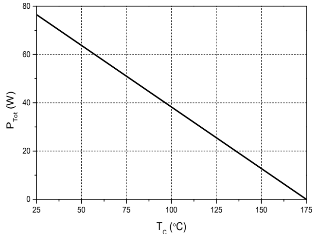
Figure 6. Power Derating
