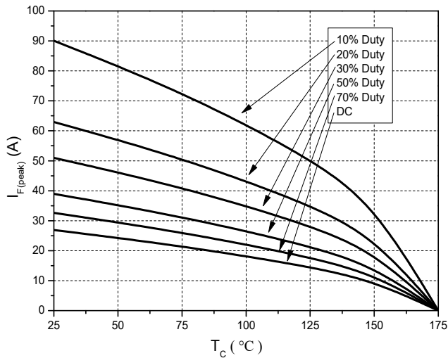
Figure 7. Current Derating
