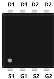
DFN3*3-D
