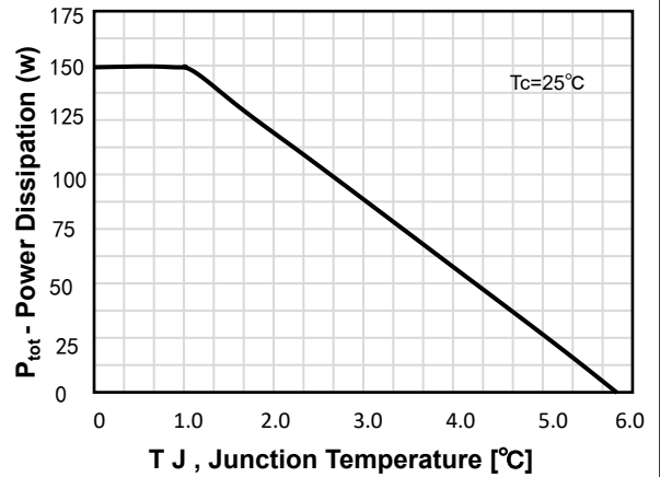
Figure 2. Power Dissipation vs Temperature
