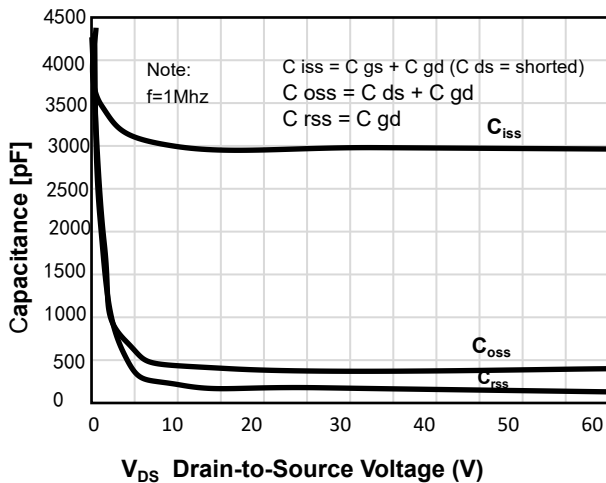
Figure 5. Capacitance Characteristics
