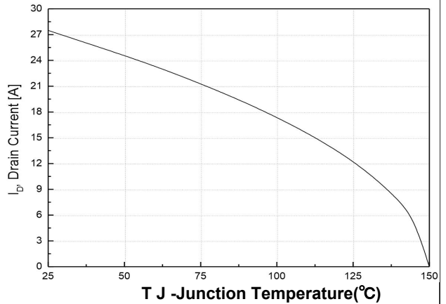
Figure 10. Maximum PContinuous Drain Current vs Case Temperature
