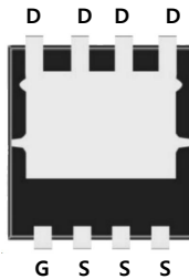
DFN5*6
